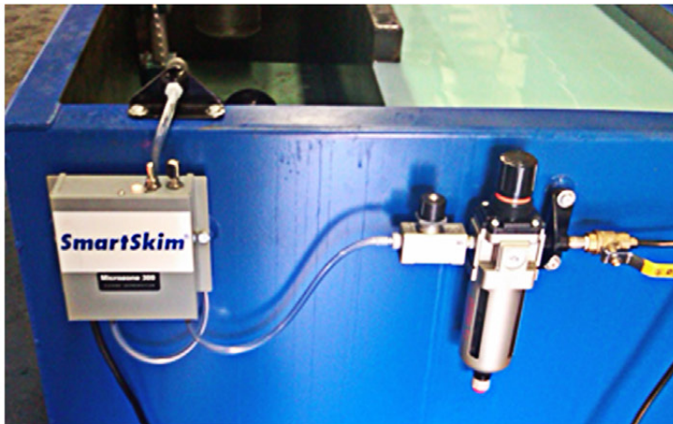
Ozone Generator on SmartSkim Coolant Recycling System
